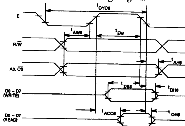
68 series timing diagram
