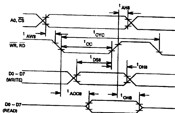
80 series timing diagram
